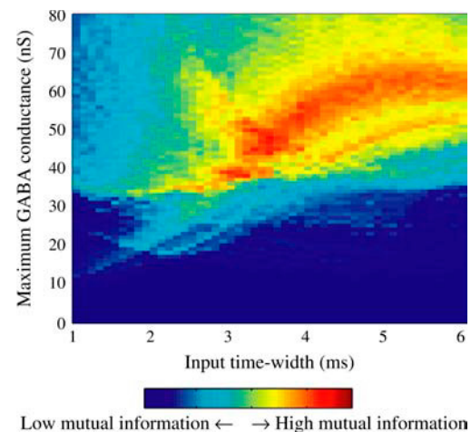
FIGURE 7 The mutual information (see Methods for details) between the input phase difference and the output firing rate for various input time-widths (the horizontal axis) and maximum amplitudes of the GABAergic inputs (the vertical axis). The period of the inputs is fixed to T = 25 (ms), and the maximum amplitude of the glutamatergic inputs are fixed to \tilde{g}_{\text{Glu}} = 9.425 (nS), which gives a 1:2 phase-locked response, i.e., 20 Hz firing in the absence of GABAergic inputs.
